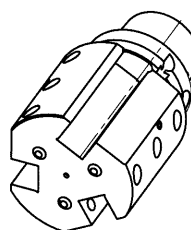
Axial toolholder 25x25 mm 142-21605 (left) 142-11605 (right)
