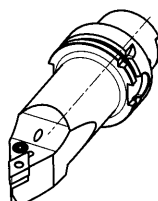
PDNNR H63APDNNR15-L145
