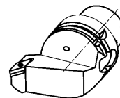
SVJB H63ASVJBL/R16-OM
