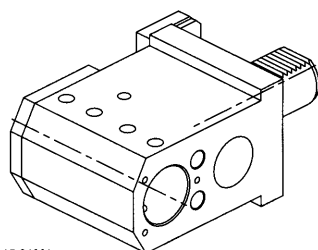
Combi toolholder for boring bar and insertdrill ø40 mm
