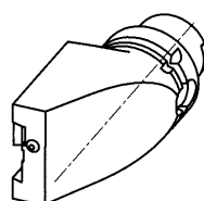
Axial toolholder for cut off tools 147-51405 (26mm, left) 147-51406 (26mm, right) 147-51407 (32mm, left) 147-51408 (32mm, right)
