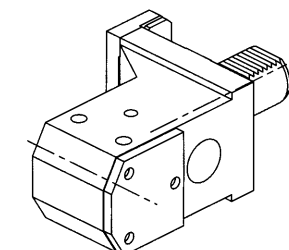
Combi toolholder for boring bar and insertdrill ø40 mm
