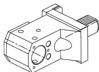
Combi toolholder for boring bar and insertdrill ø40 mm
